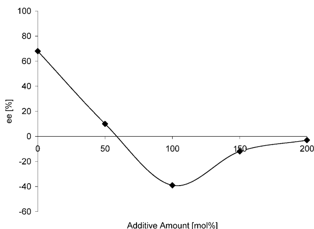
Figure 5. The ee value of 3 versus amount of imidazole as additive.
