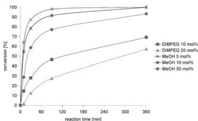
Figure 1. Kinetic study for phenyl transfer reactions in the presence of DiMPEG (MW 2000) and methanol.
