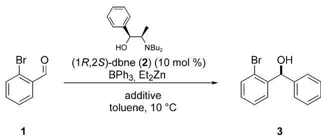
Scheme 1. Addition of phenylzinc to 2-bromobenzaldehyde ( 1 ).
