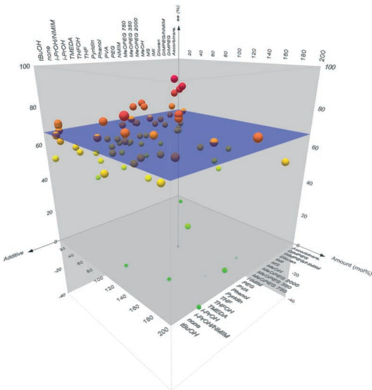
Figure 2. High-throughput screening of additives.
