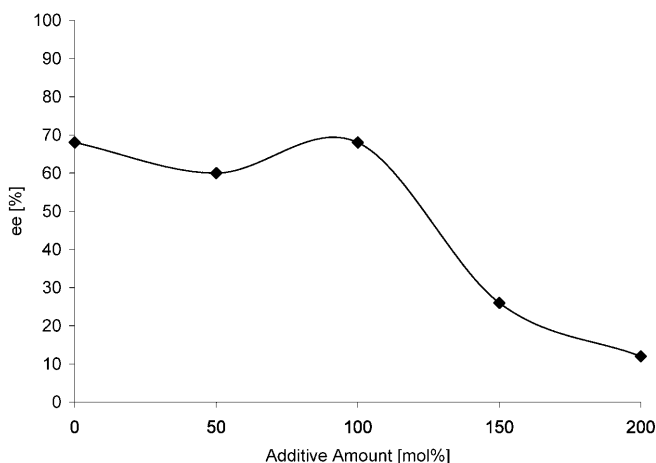
Figure 4. The ee value of 3 versus the amount of pyridine as additive.
