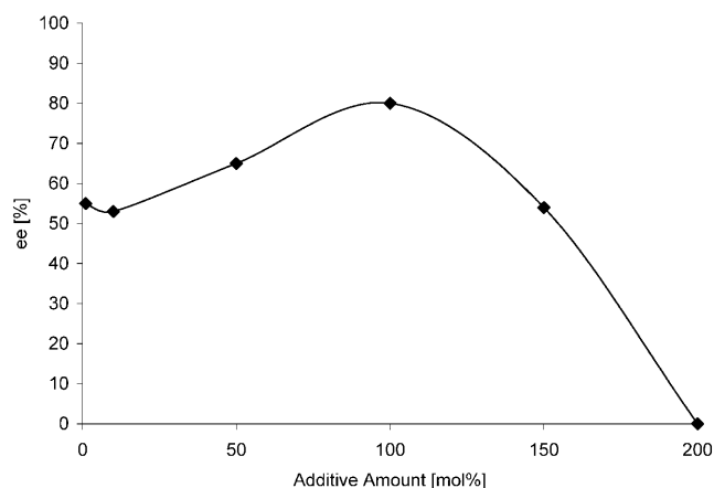
Figure 3. The ee value of 3 versus the amount of 2-propanol as additive.
